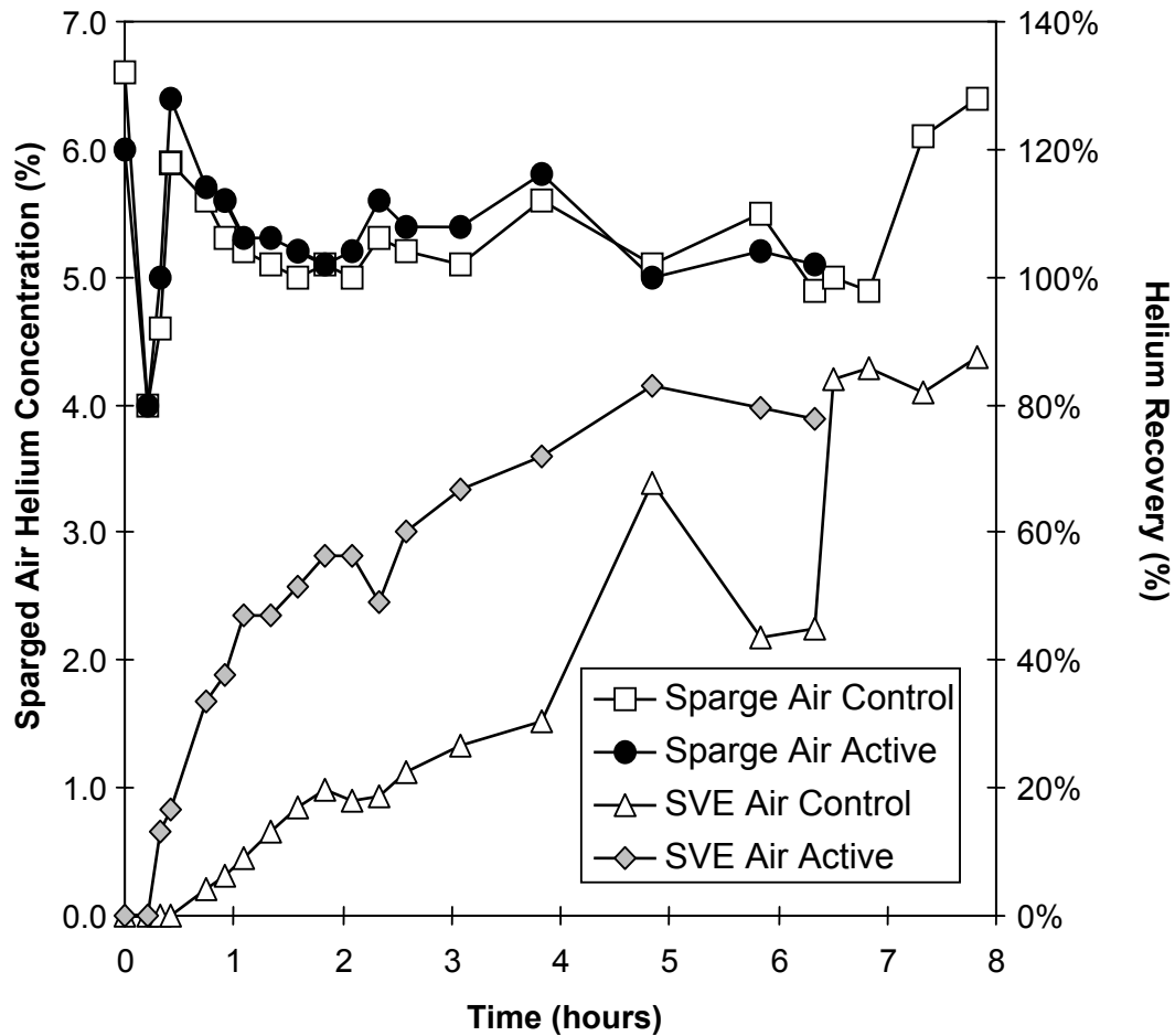
Figure 7. Helium Tracer Test Results from the Control Test Plot and the Active Test Plot
