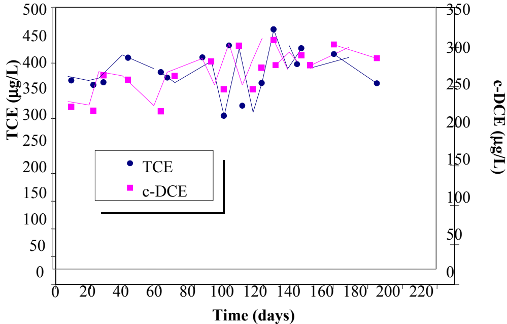
Figure 24. Control Vadose Zone Monitoring Point SG-A3-95
