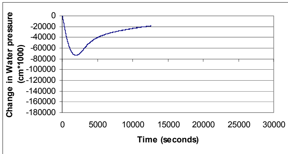
Figure 10. Water Pressure Change at MWA1 During Shutdown at the Control Test Plot
