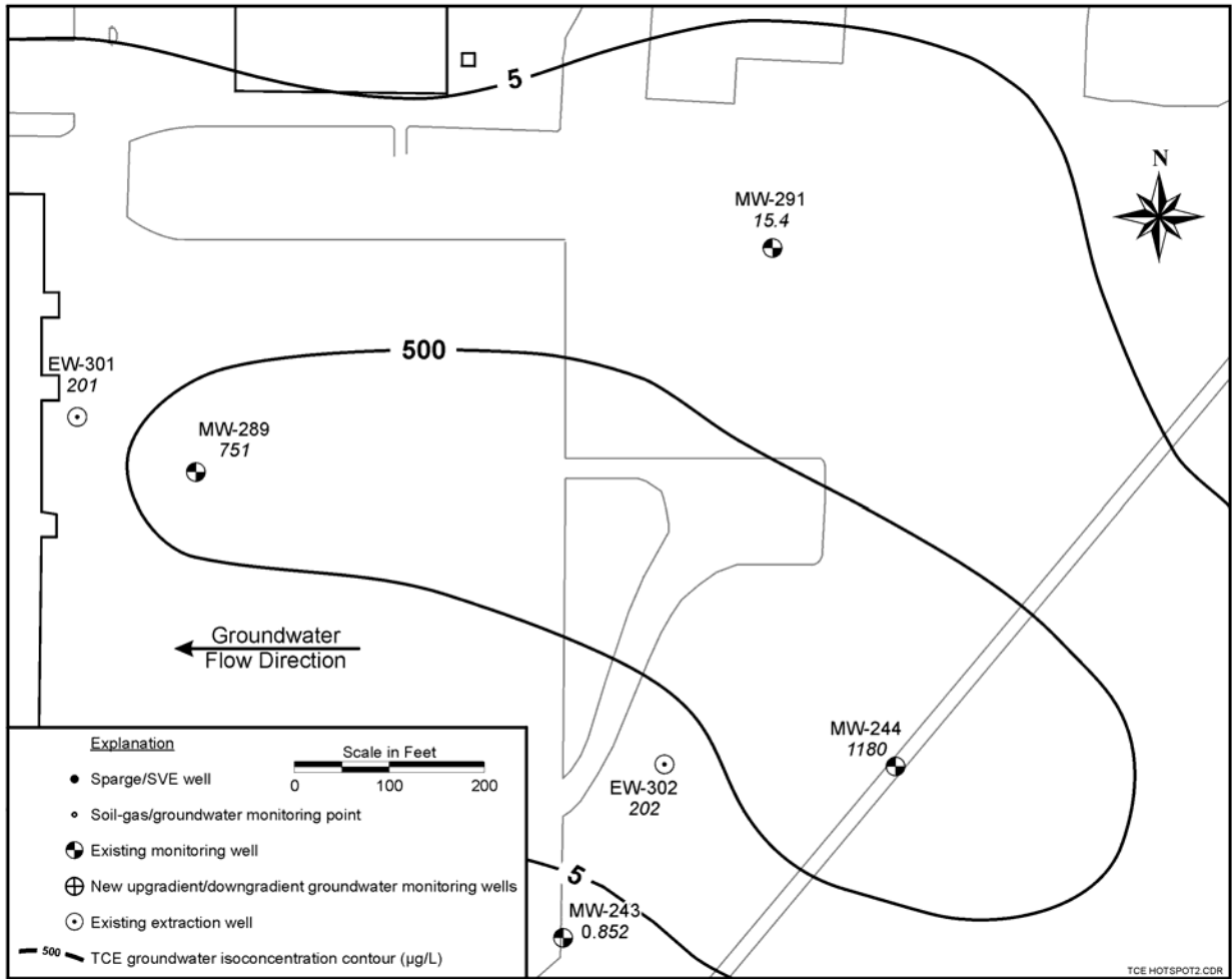
Figure 3. TCE Plume Contours at OU A
