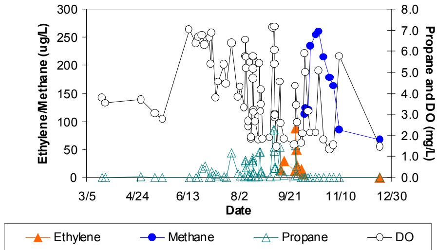
Figure 26. Concentrations of CAH Compounds and Primary Growth Substrates (Propane and Methane) in MW-C4-117 during Phase 2
