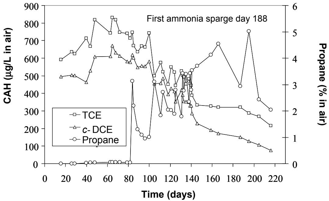
Figure 23. Vadose Zone Monitoring Point SG-C6-105
