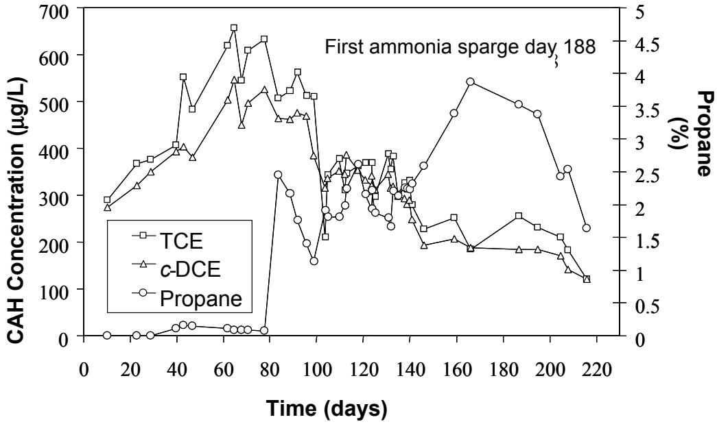
Figure 22. Vadose Zone Monitoring Point SG-C2-95
