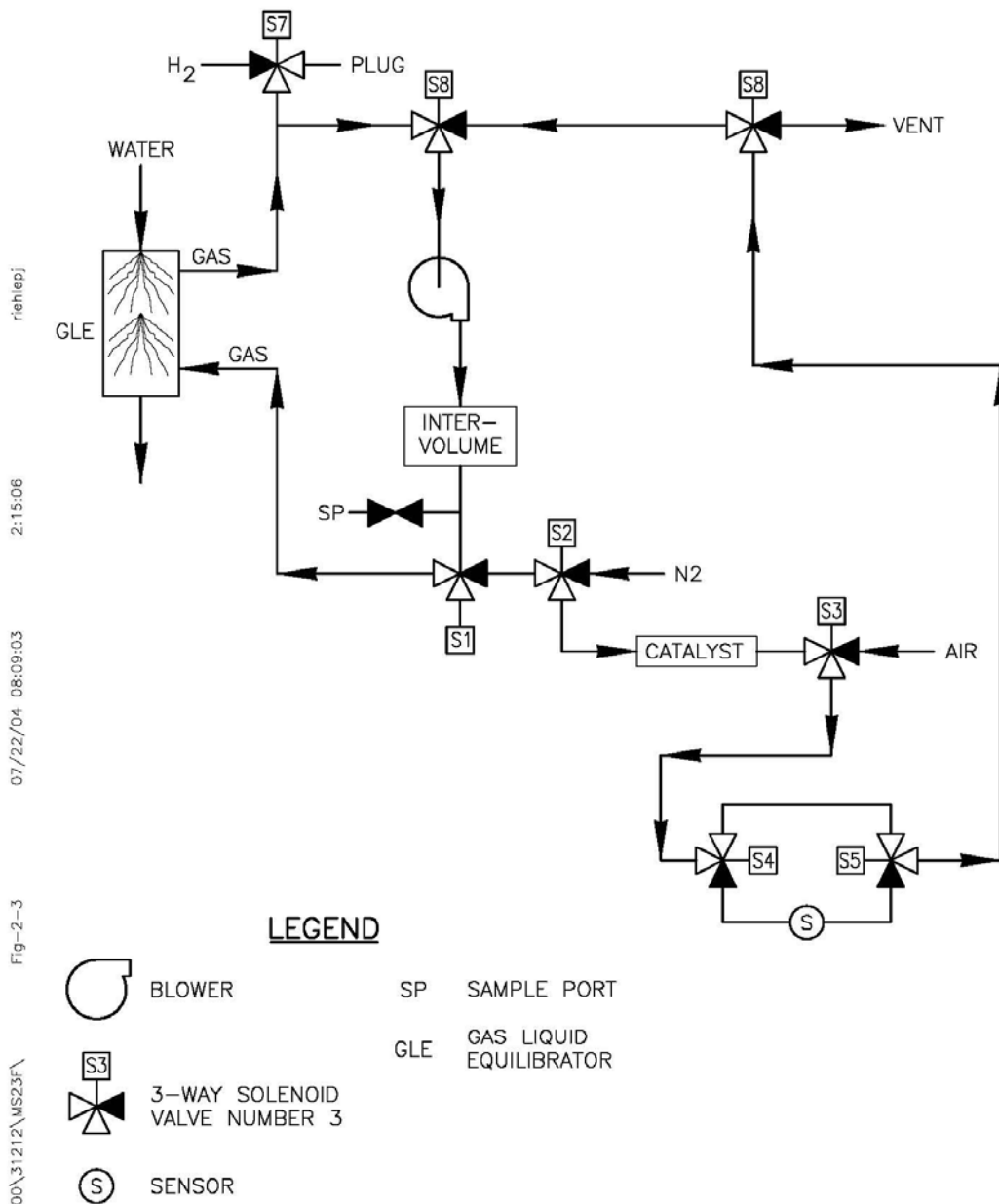
Figure 2-3 DH ANALYZER PROCESS FLOW DIAGRAM
