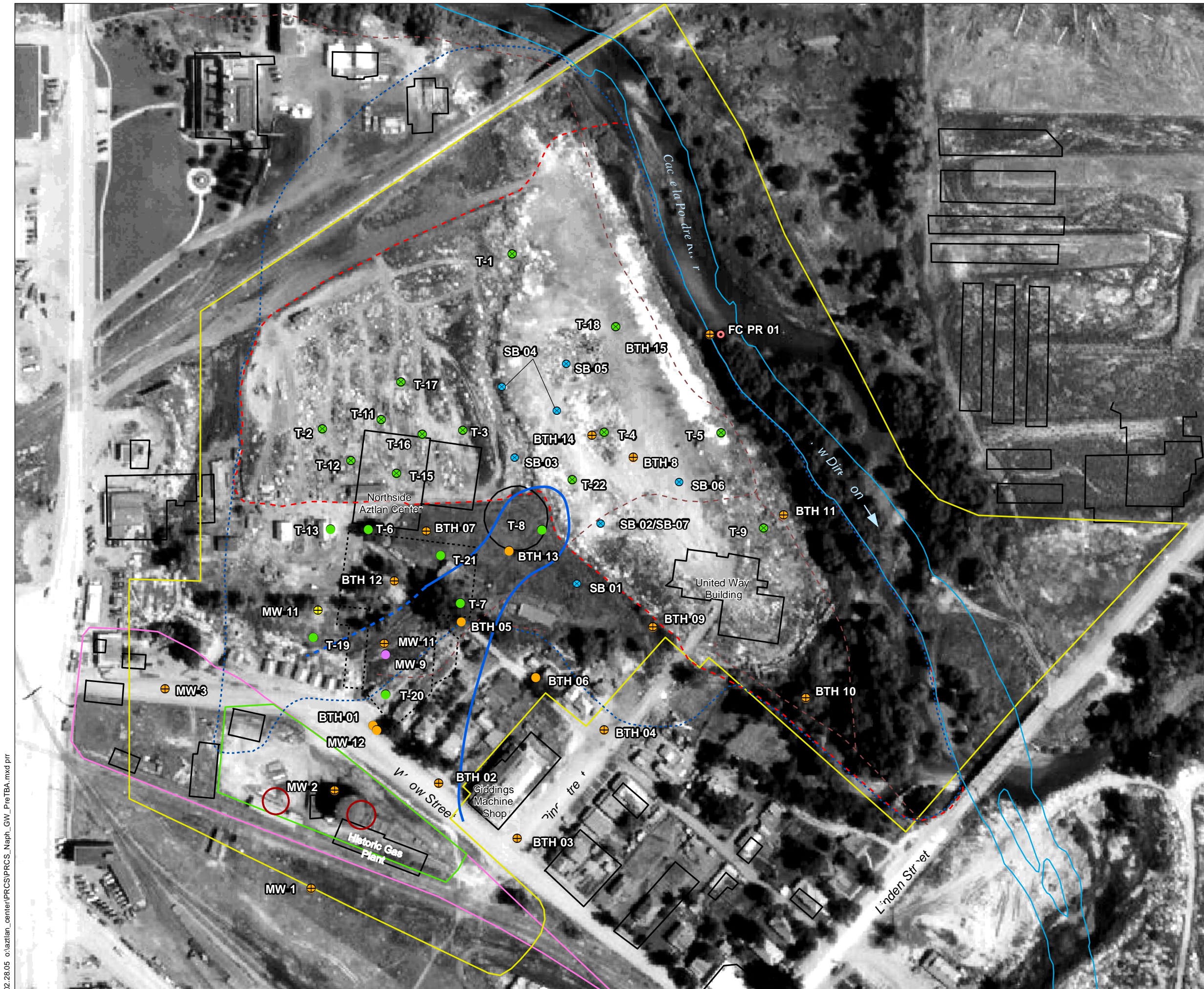
POUDRE RIVER SITE FORT COLLINS, COLORADO FIGURE 7 NAPHTHALENE CONCENTRATIONS IN GROUNDWATER, PRE-TBA U.S. EPA REGION VIII IN COOPERATION WITH BROWNFIELDS TECHNOLOGY SUPPORT CENTER AND TETRA TECH EM, INC.
