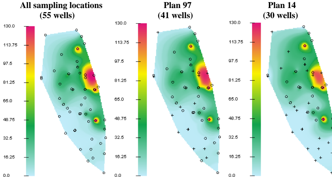
Figure 5-2. Example of Plume Maps for Plans Selected from Tradeoff Curve
