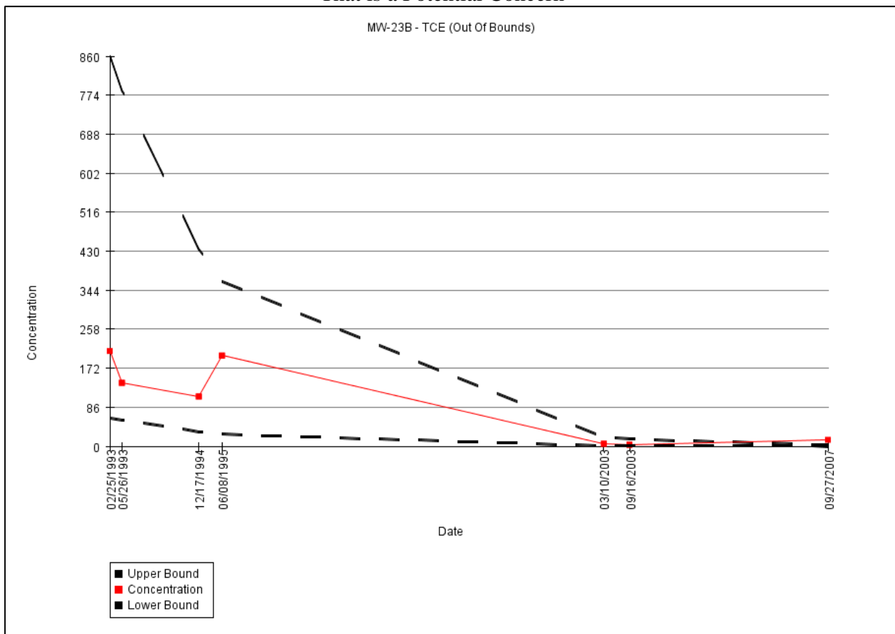
Figure 5-3. Example Data Tracker Plot With “Out-of-Bounds” Value That is a Potential Concern
