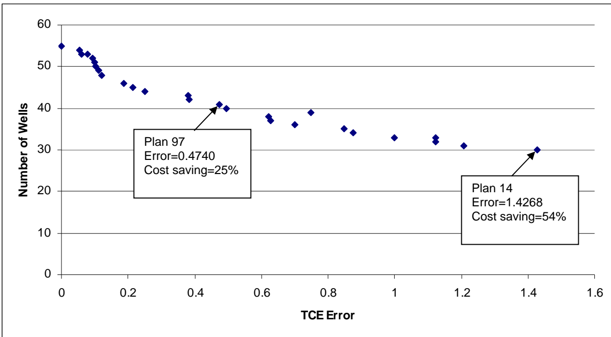
Figure 5-1. Example Tradeoff Curve for Spatial Redundancy Evaluation, GAFB Site
