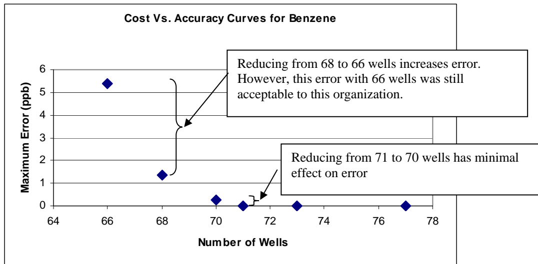
Figure 2-2. Example of a Tradeoff Curve for Spatial Optimization
