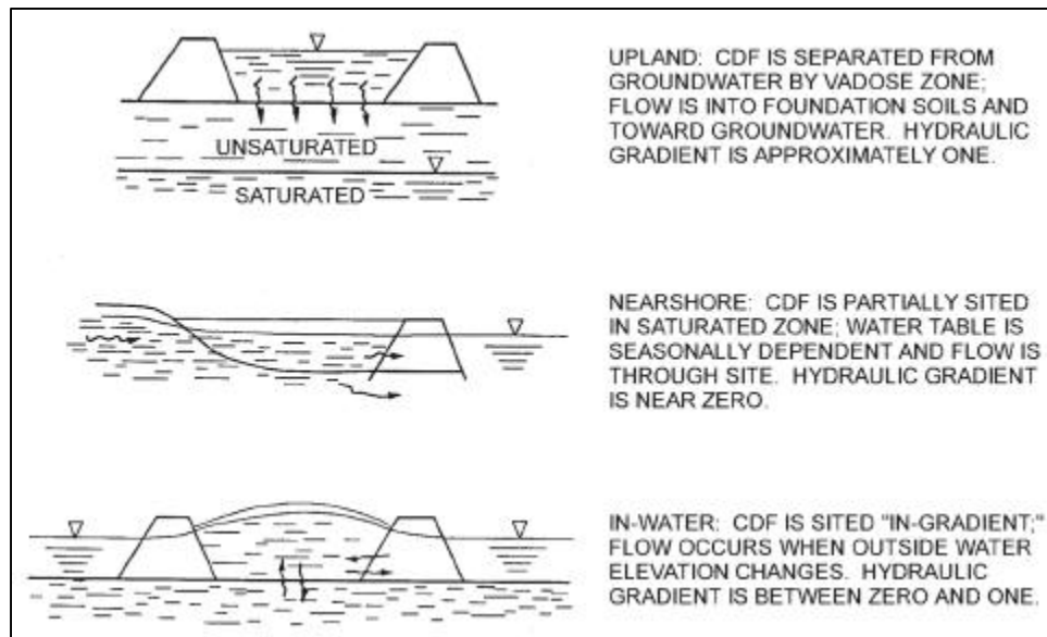
Figure 6-1. Illustration of potential CDF leachate pathways
