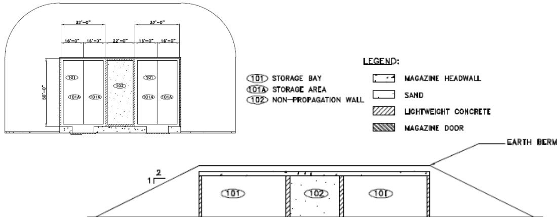
FIGURE 4-2. HP-2B PLAN VIEW/CROSS-SECTION
