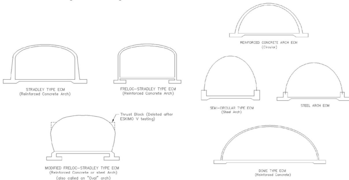
FIGURE 4-1. ECM CROSS-SECTIONS
