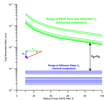
Graphical comparison of pore gas velocities and diffusion rates.
