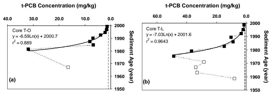
Vertical profile showing surface sediment recovery in two PCB-contaminated Lake Hartwell sediment cores. Solid symbols represent data used to generate the curves. Reprinted with permission from Brenner et al., 2004. Copyright 2004 American Chemical Society.
