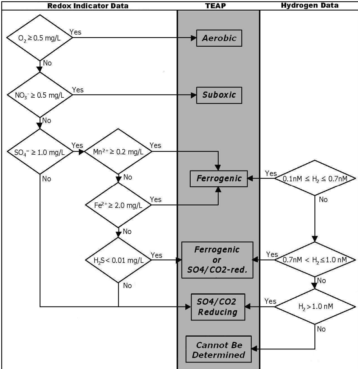
Figure 38. Flow Chart for Determining Redox Conditions
